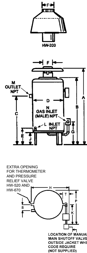
FIGURE 1. DIMENSIONS
