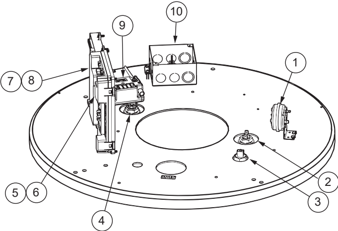
Figure 9. Inner Cover Control Assembly - 100 Gallon
