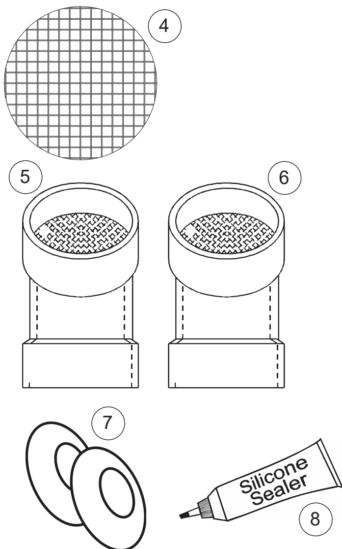
Figure 15. 3" Vent Kits
