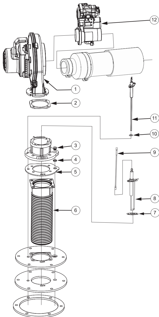
Figure 12. 100-Gallon Gas Valve/Blower/Burner Assembly
