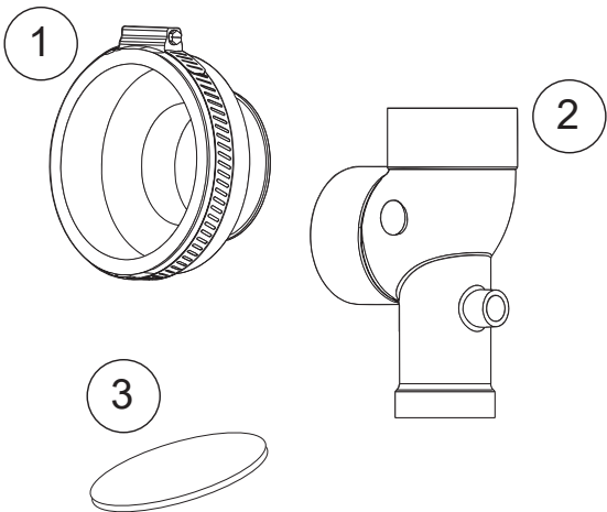
Figure 16. 4" Exhaust Connector Kits
